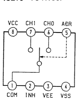
IC216 TC4W53F
