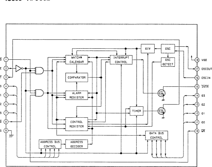
IC303 RF5C62
