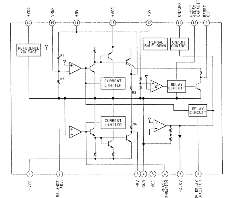
IC509 M5294P
