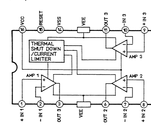
IC404, 405 LA6523
