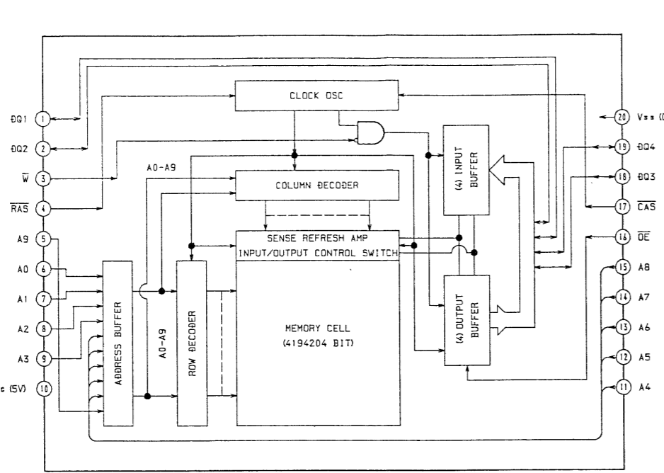
IC109 M5U44400
