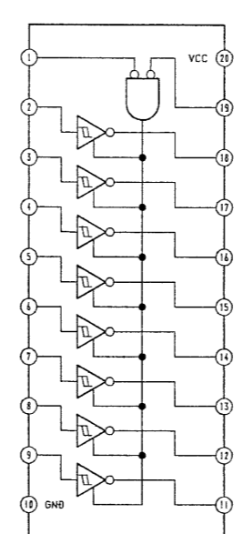
IC401 TC74ATC540F
