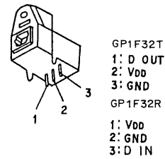
GP1F32R GP1F32T
