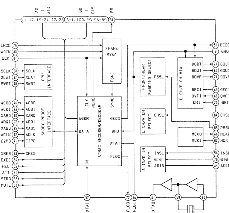
IC101 CXD2527R
