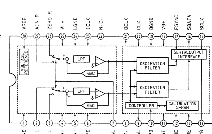
IC510 CS5339-KS
