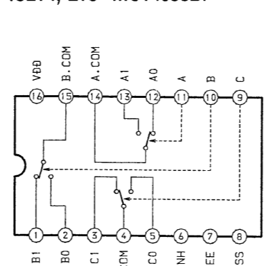
IC214, 215 MC14053BF
