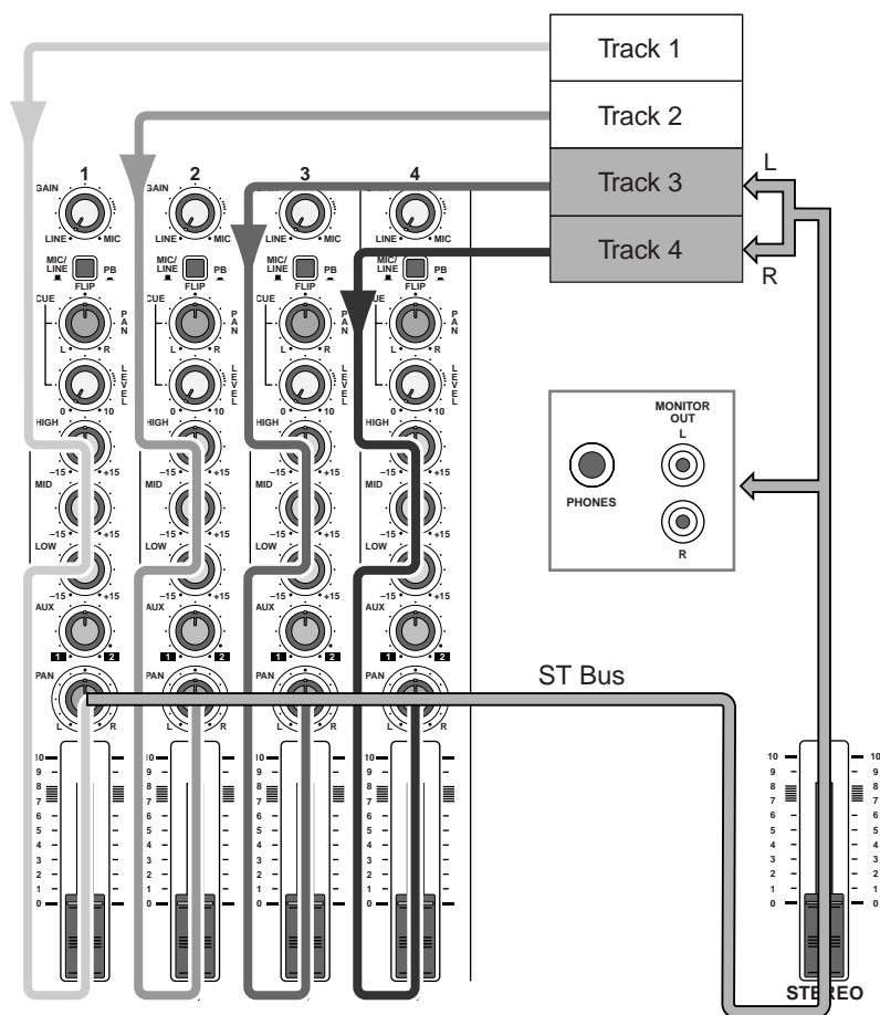
Signal flow for ping-pong recording
